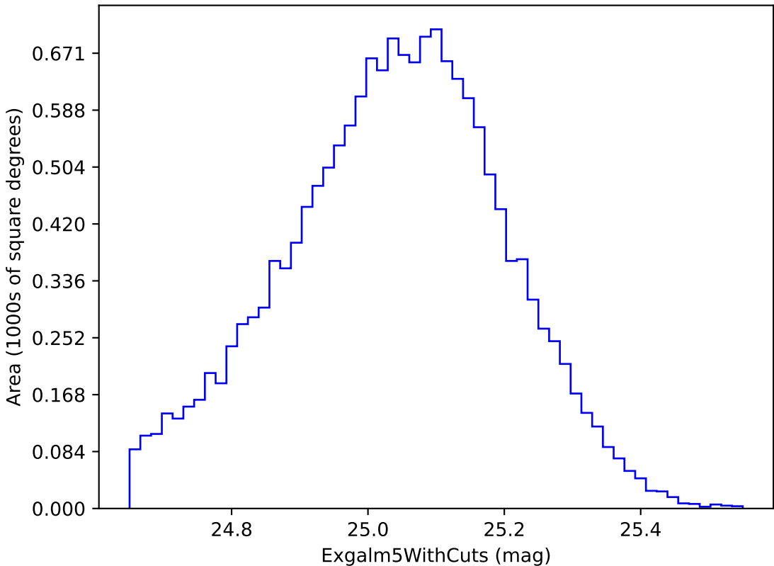
baseline_v2.0_10yrs i band non-DD year 1: ExgalM5WithCuts
