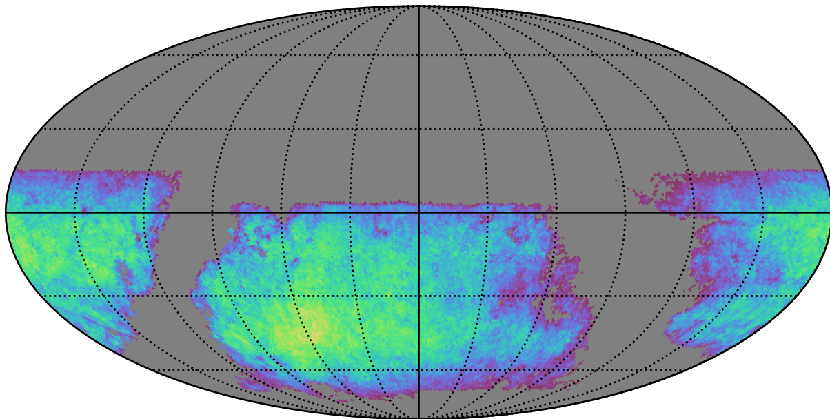
baseline_v2.0_10yrs i band non-DD year 10: ExgalM5WithCuts
