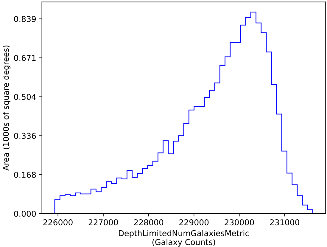
baseline_v2.0_10yrs i band galaxies non-DD: DepthLimitedNumGalaxiesMetric
