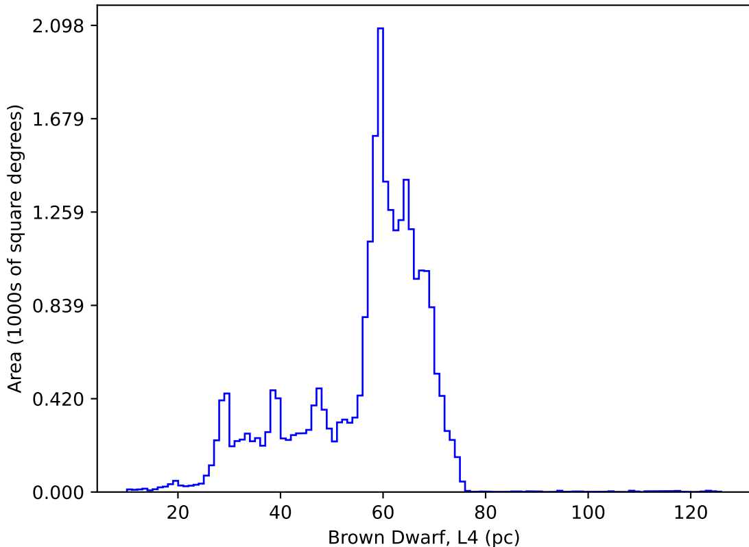
baseline_v2.0_10yrs : Brown Dwarf, L4
