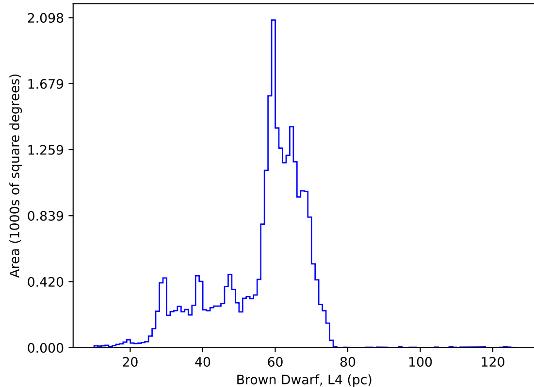
baseline_v2.0_10yrs : Brown Dwarf, L4
