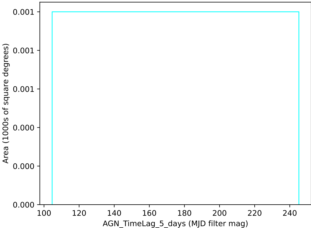
baseline_v2.0_10yrs u band: AGN_TimeLag_5_days
