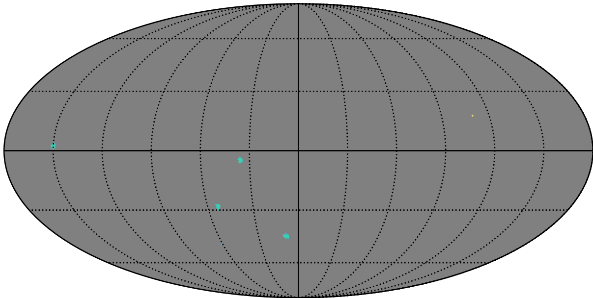
baseline_v2.0_10yrs r band: AGN_TimeLag_5_days
