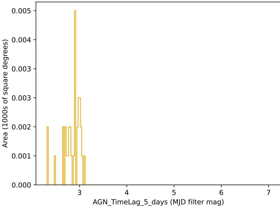
baseline_v2.0_10yrs r band: AGN_TimeLag_5_days
