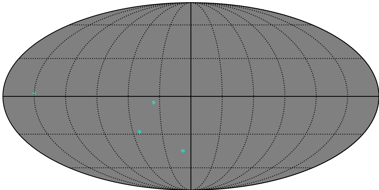
baseline_v2.0_10yrs i band: AGN_TimeLag_5_days
