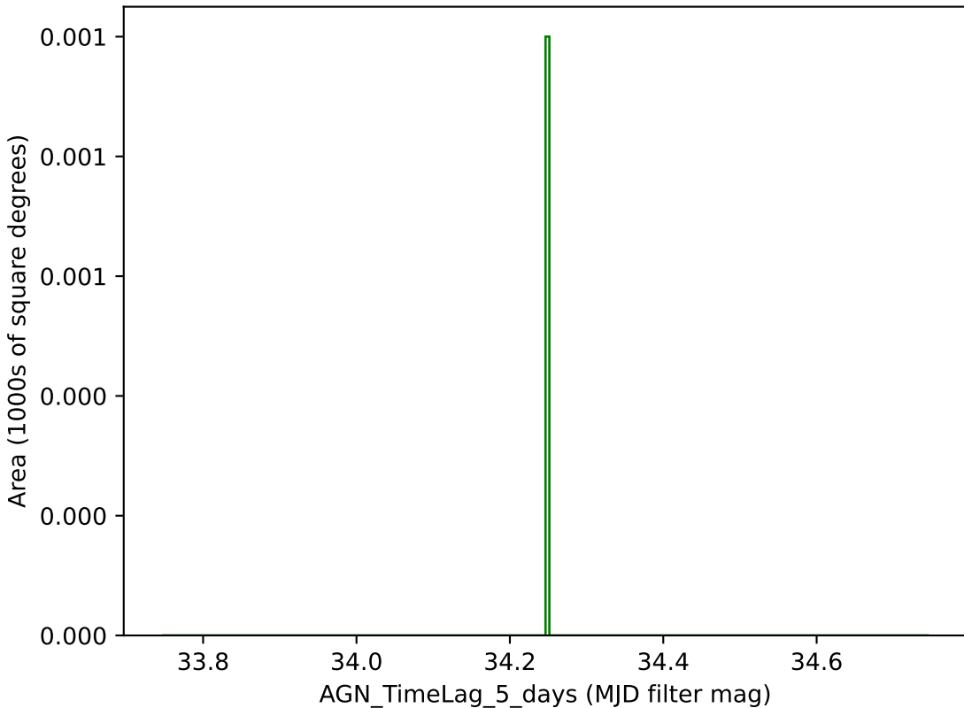
baseline_v2.0_10yrs g band: AGN_TimeLag_5_days
