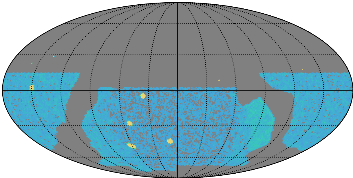
baseline_v2.0_10yrs z band: AGN_TimeLag_100_days
