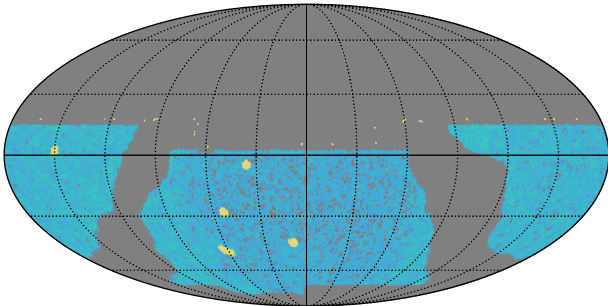
baseline_v2.0_10yrs y band: AGN_TimeLag_100_days
