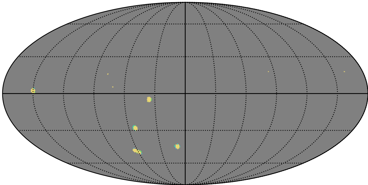
baseline_v2.0_10yrs u band: AGN_TimeLag_100_days
