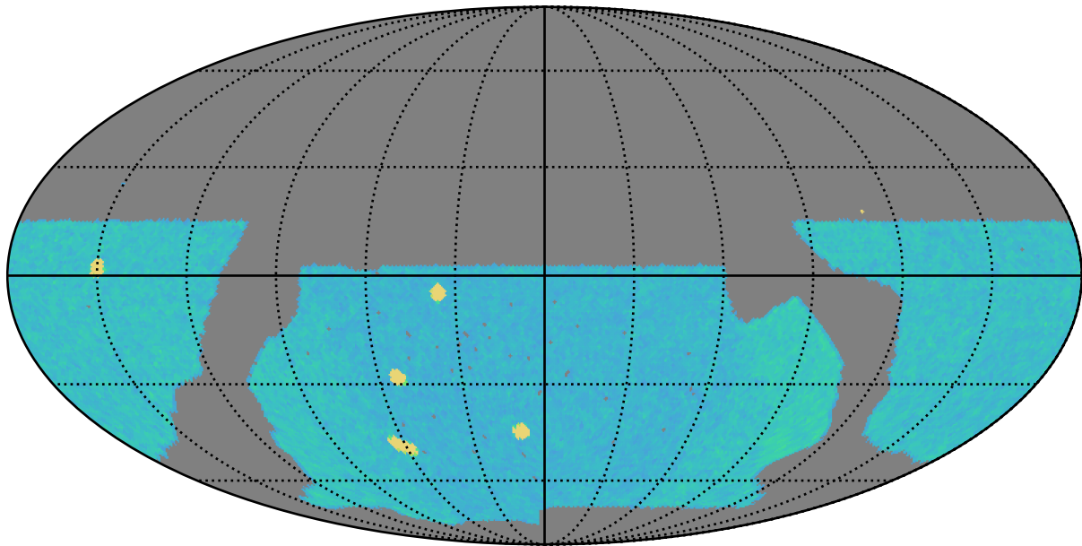
baseline_v2.0_10yrs r band: AGN_TimeLag_100_days
