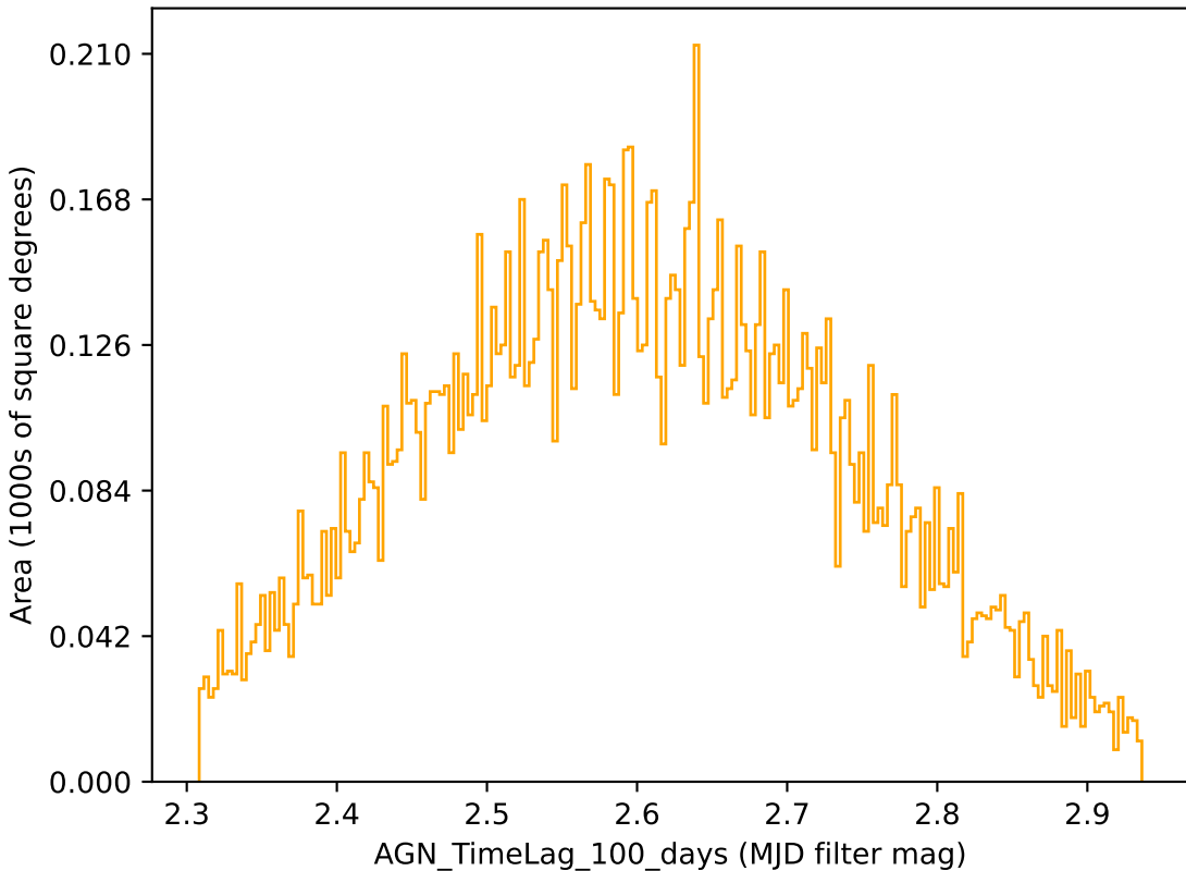
baseline_v2.0_10yrs r band: AGN_TimeLag_100_days
