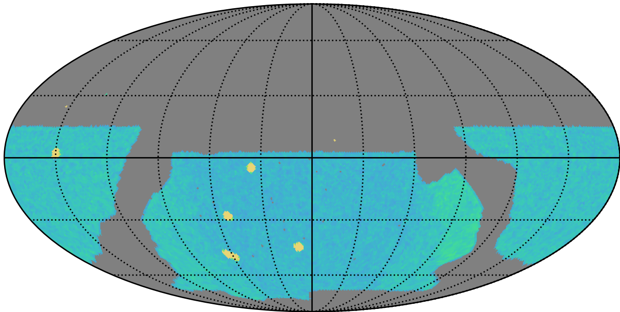
baseline_v2.0_10yrs i band: AGN_TimeLag_100_days
