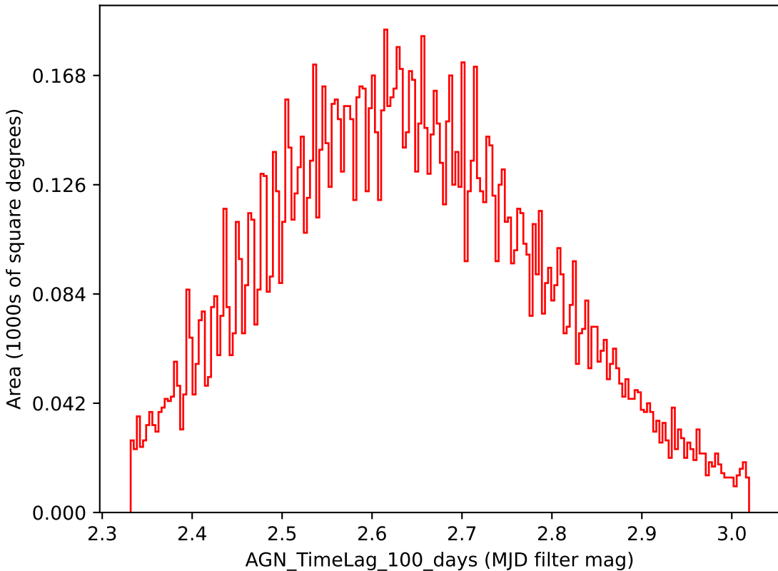
baseline_v2.0_10yrs i band: AGN_TimeLag_100_days
