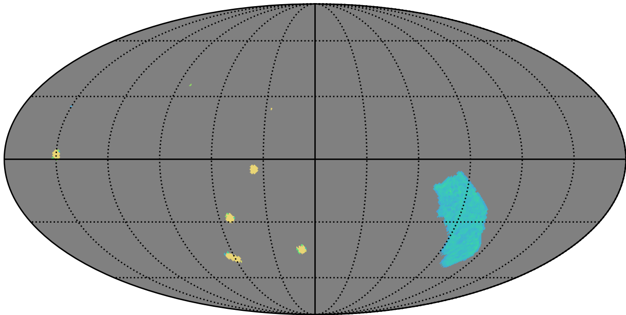
baseline_v2.0_10yrs g band: AGN_TimeLag_100_days
