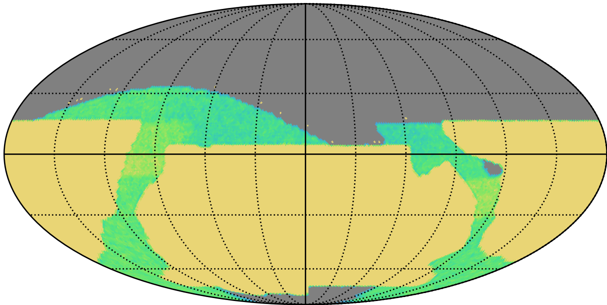
baseline_v2.0_10yrs all bands: AGN_TimeLag_100_days
