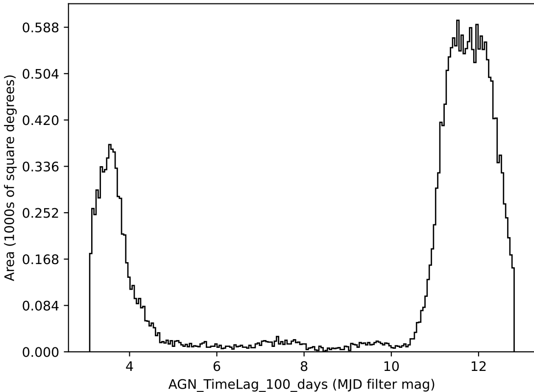
baseline_v2.0_10yrs all bands: AGN_TimeLag_100_days
