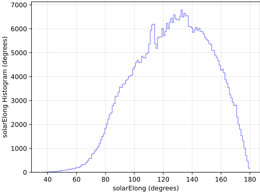
baseline_v2.0_10yrs WFD r band: solarElong Histogram
