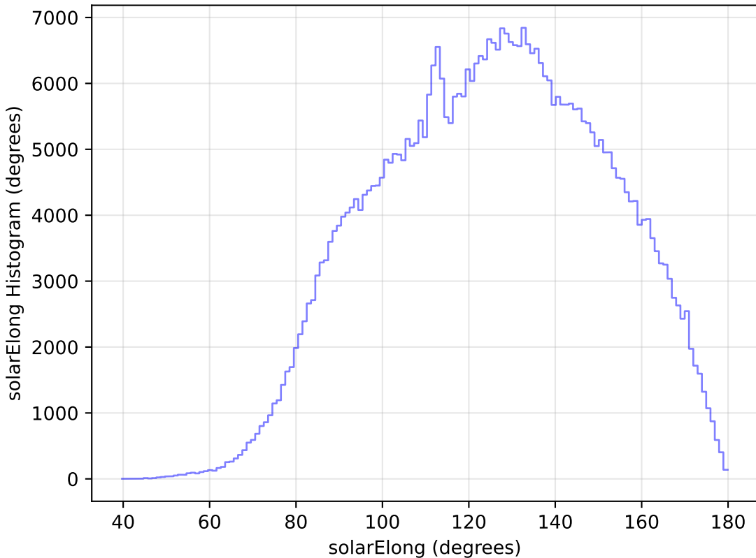
baseline_v2.0_10yrs WFD i band: solarElong Histogram
