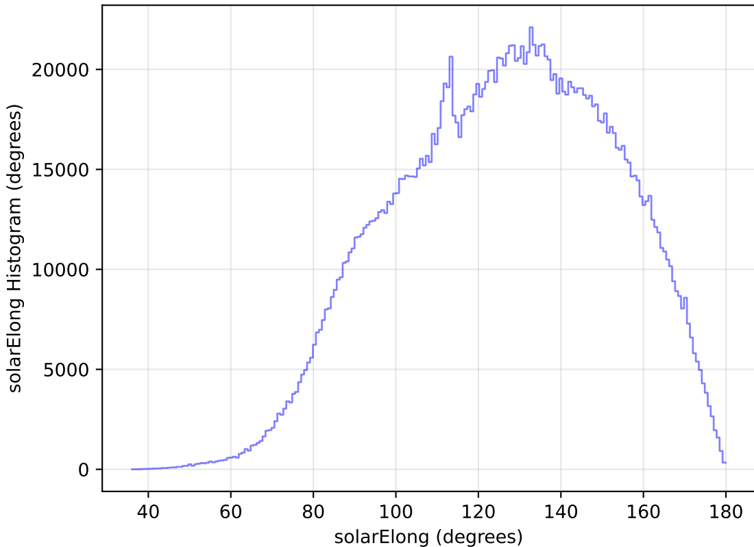
baseline_v2.0_10yrs WFD all bands: solarElong Histogram
