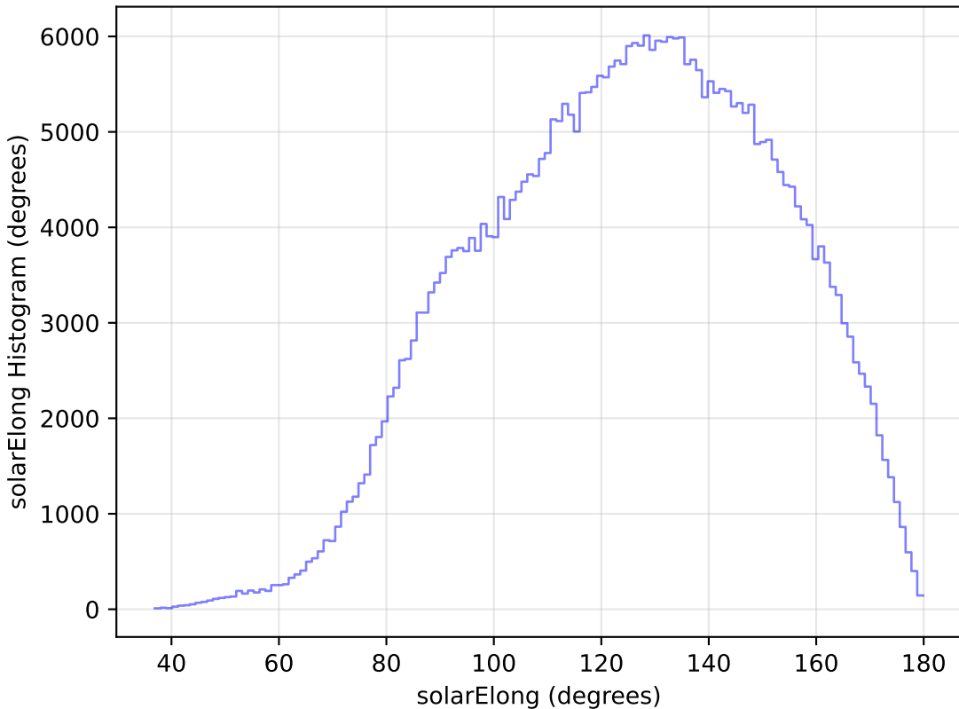
baseline_v2.0_10yrs All sky z band: solarElong Histogram
