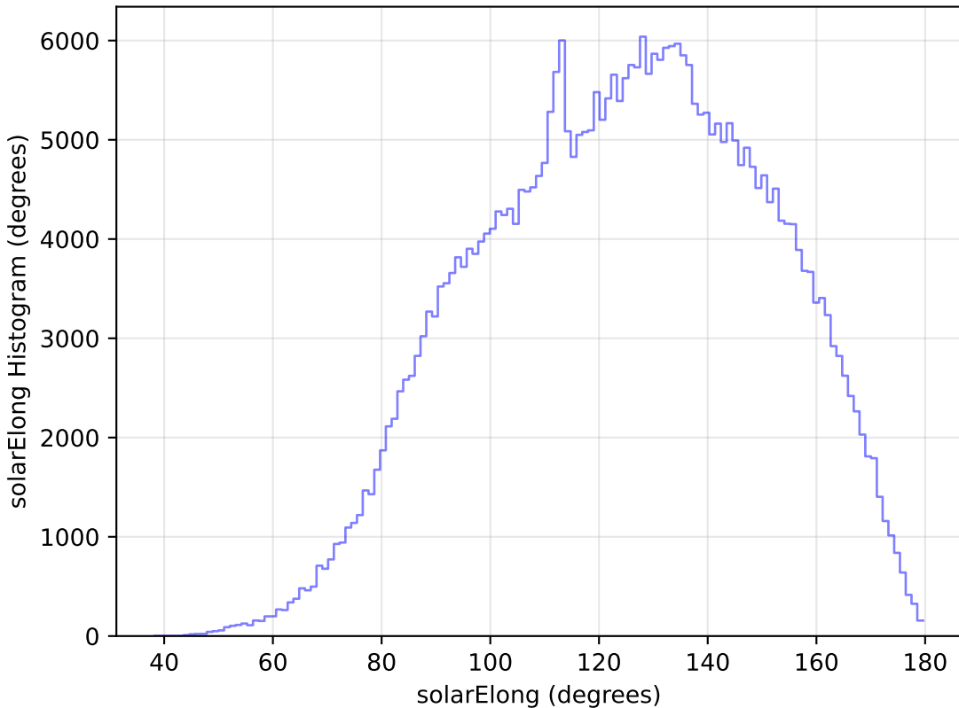
baseline_v2.0_10yrs All sky y band: solarElong Histogram
