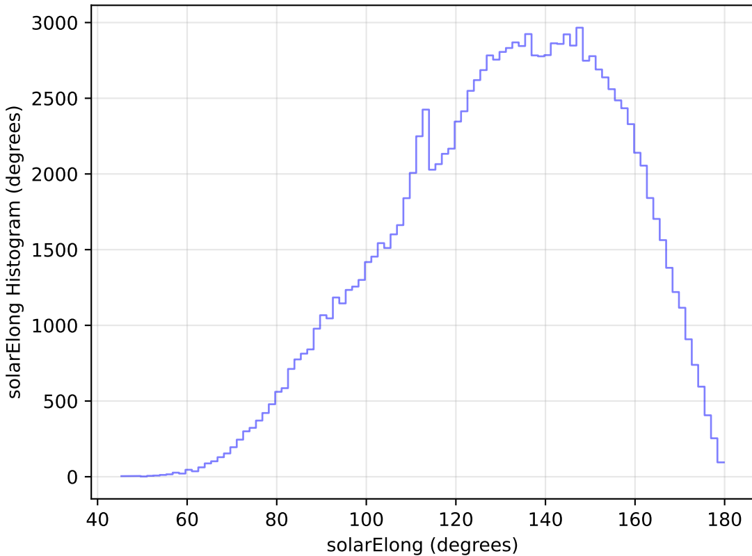
baseline_v2.0_10yrs All sky u band: solarElong Histogram
