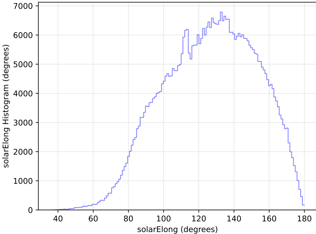
baseline_v2.0_10yrs All sky r band: solarElong Histogram
