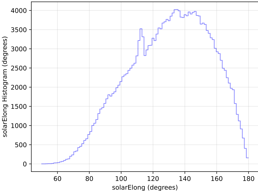
baseline_v2.0_10yrs All sky g band: solarElong Histogram
