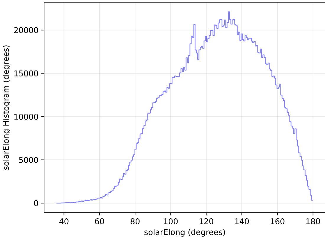
baseline_v2.0_10yrs All sky all bands: solarElong Histogram
