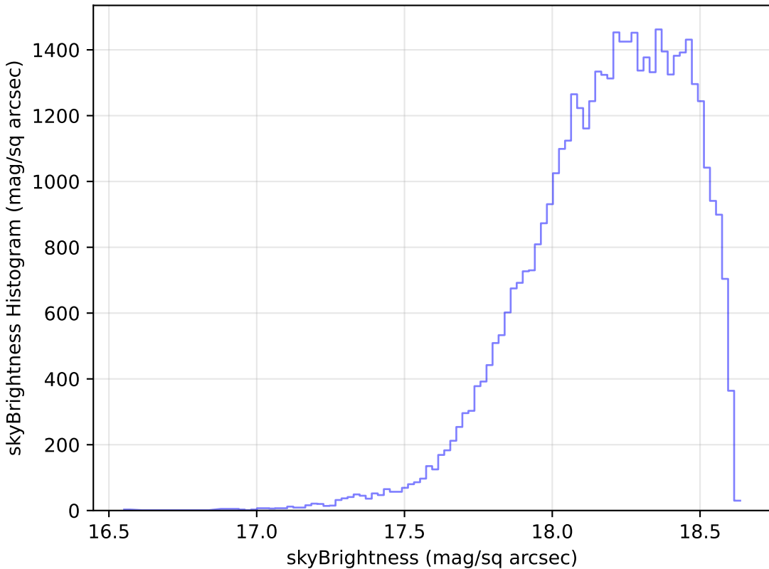
baseline_v2.0_10yrs Yr 1 y band: skyBrightness Histogram
