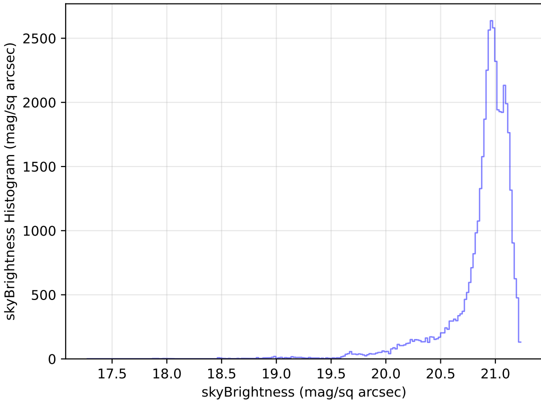
baseline_v2.0_10yrs Yr 1 r band: skyBrightness Histogram
