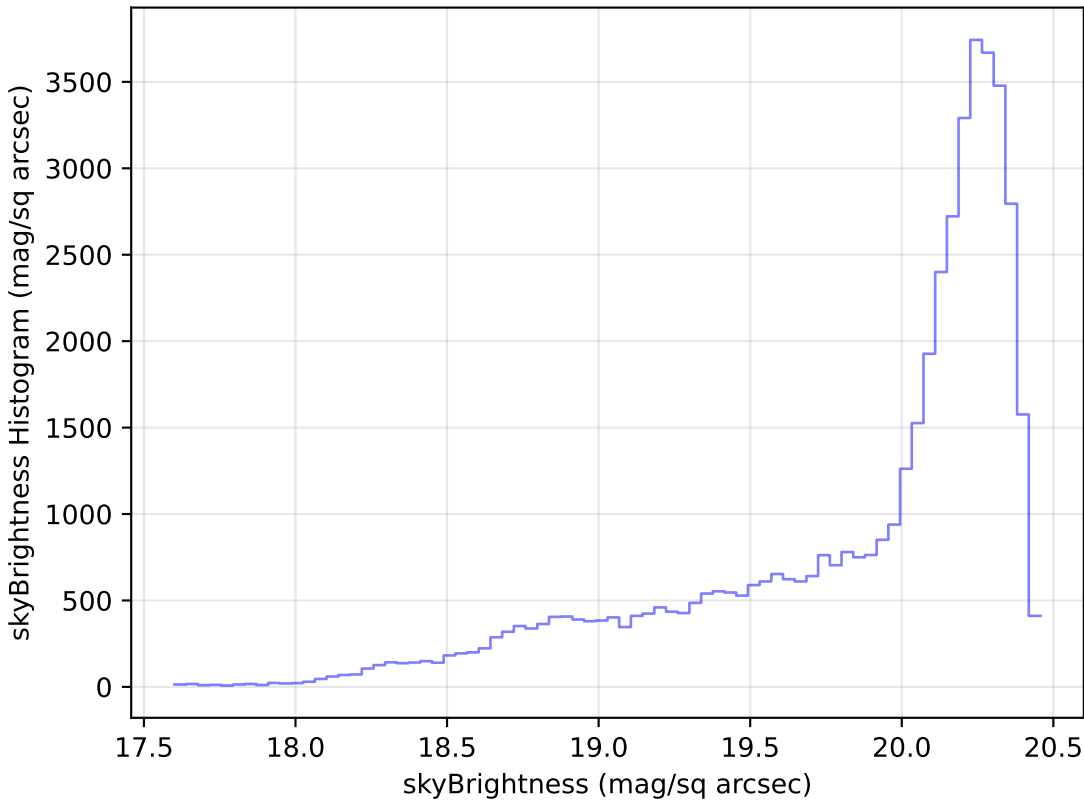
baseline_v2.0_10yrs Yr 1 i band: skyBrightness Histogram
