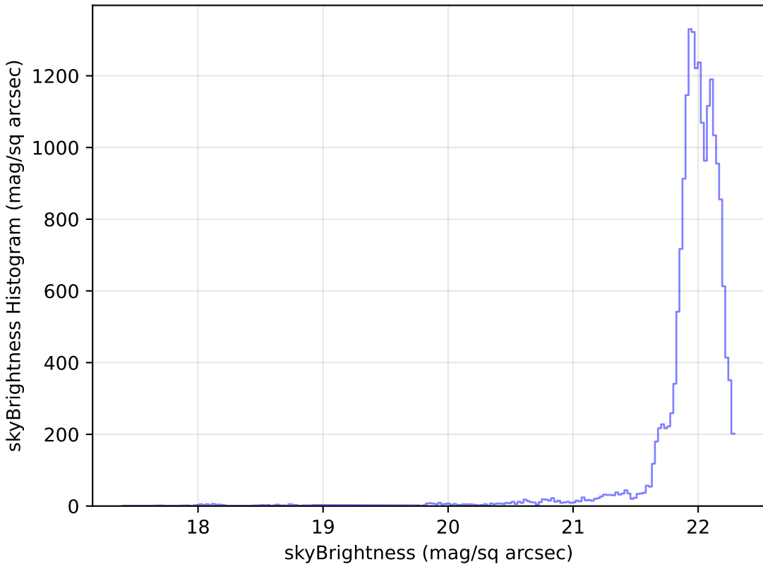
baseline_v2.0_10yrs Yr 1 g band: skyBrightness Histogram
