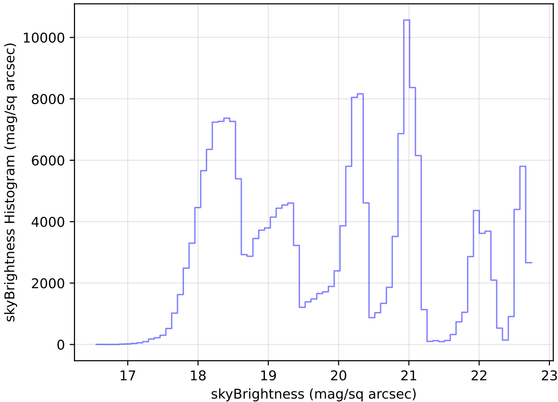
baseline_v2.0_10yrs Yr 1 all bands: skyBrightness Histogram
