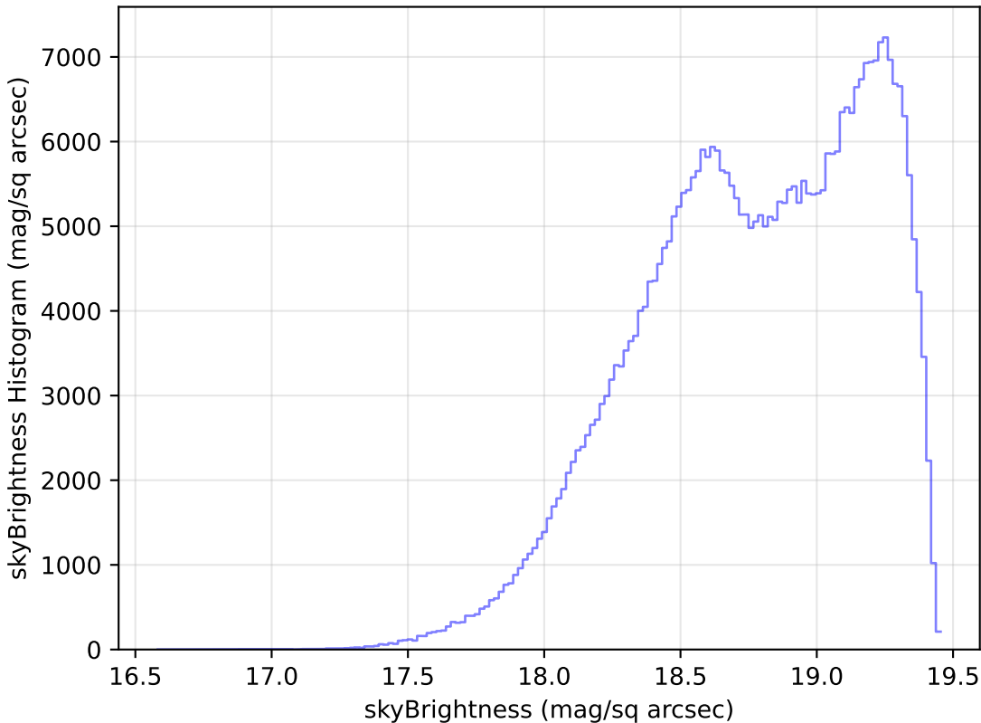
baseline_v2.0_10yrs WFD z band: skyBrightness Histogram
