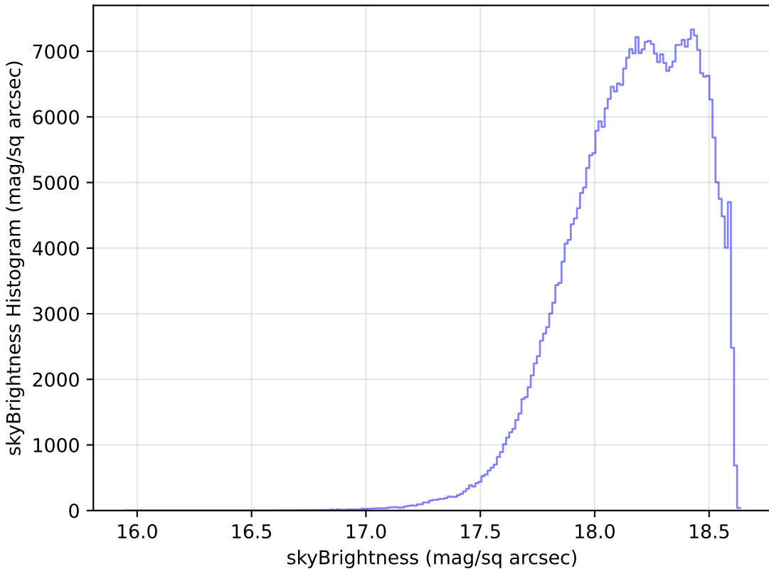
baseline_v2.0_10yrs WFD y band: skyBrightness Histogram
