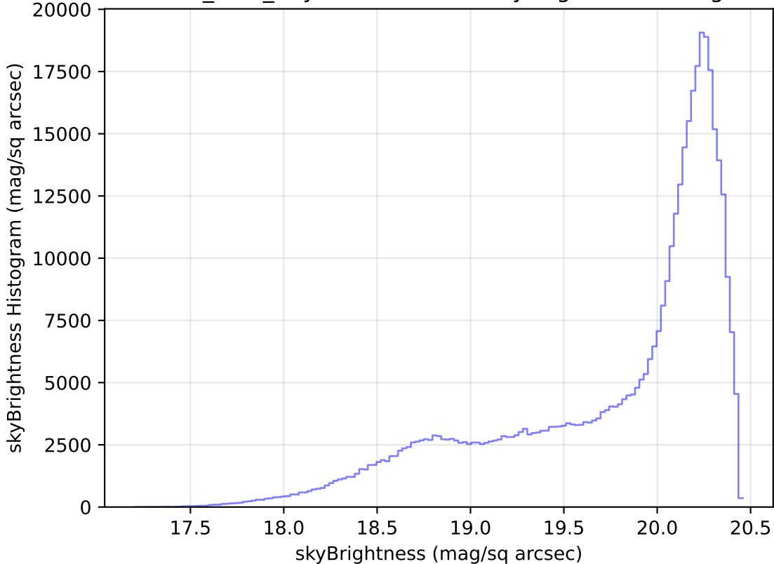
baseline_v2.0_10yrs WFD i band: skyBrightness Histogram
