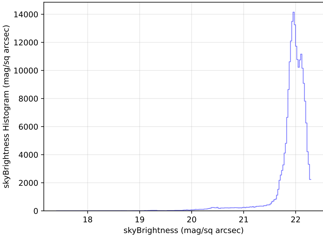
baseline_v2.0_10yrs WFD g band: skyBrightness Histogram
