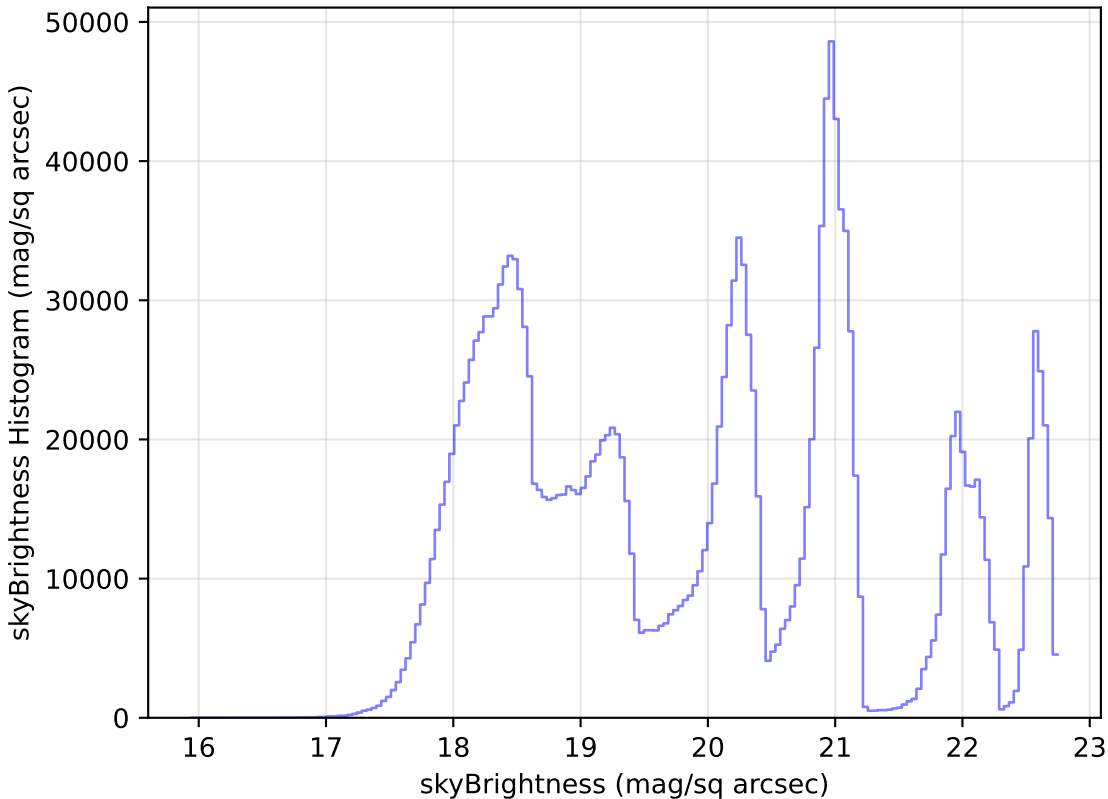
baseline_v2.0_10yrs WFD all bands: skyBrightness Histogram
