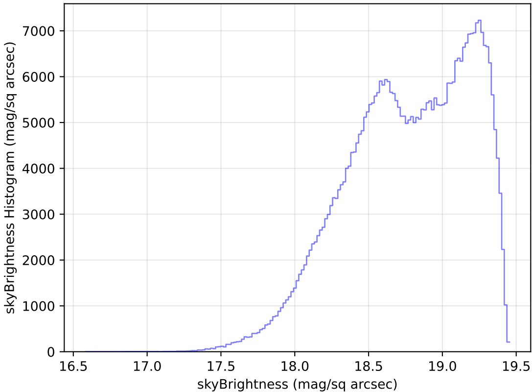
baseline_v2.0_10yrs All sky z band: skyBrightness Histogram
