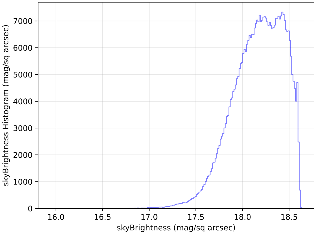
baseline_v2.0_10yrs All sky y band: skyBrightness Histogram
