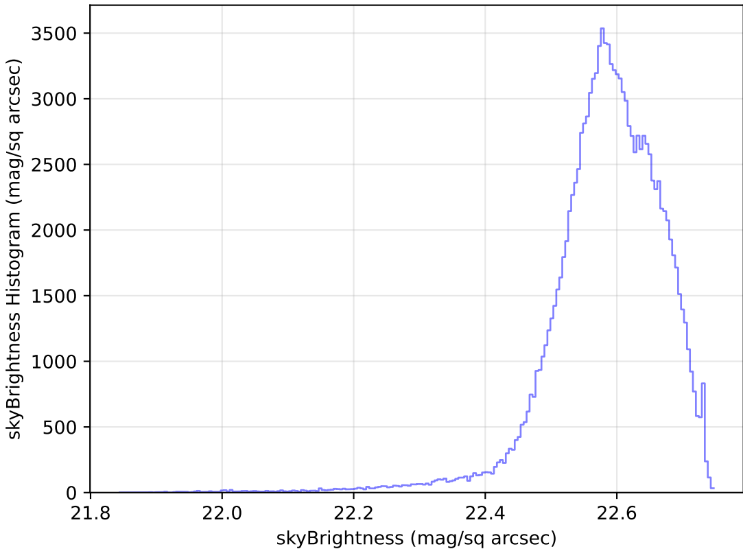
baseline_v2.0_10yrs All sky u band: skyBrightness Histogram
