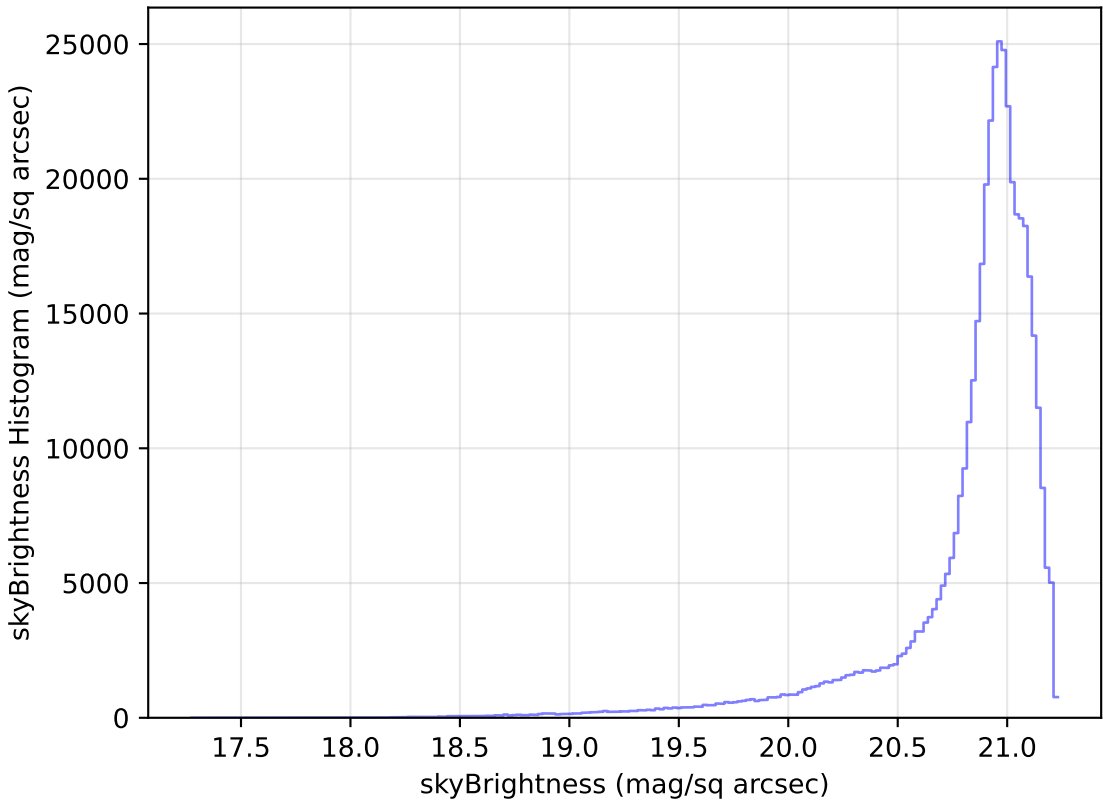
baseline_v2.0_10yrs All sky r band: skyBrightness Histogram
