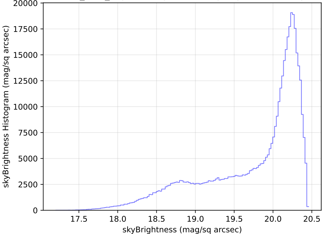
baseline_v2.0_10yrs All sky i band: skyBrightness Histogram
