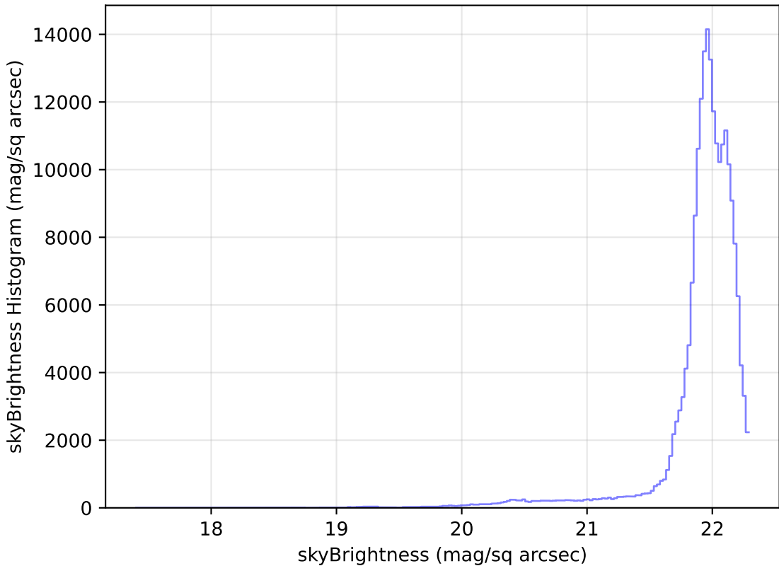
baseline_v2.0_10yrs All sky g band: skyBrightness Histogram
