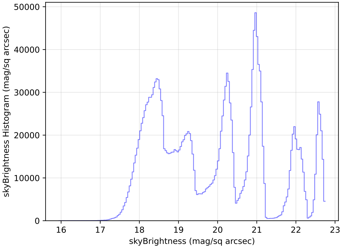
baseline_v2.0_10yrs All sky all bands: skyBrightness Histogram
