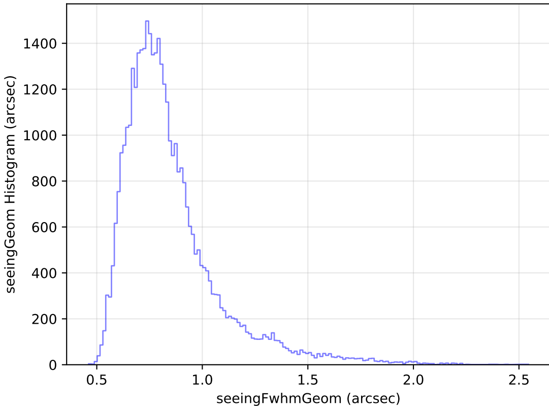
baseline_v2.0_10yrs Yr 1 z band: seeingGeom Histogram
