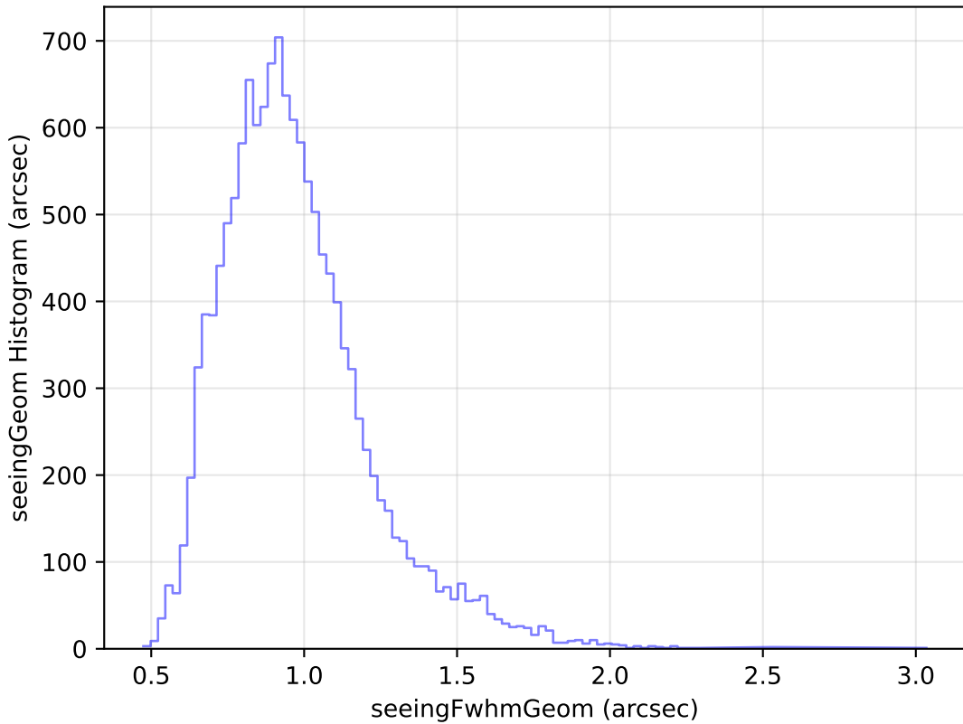
baseline_v2.0_10yrs Yr 1 u band: seeingGeom Histogram
