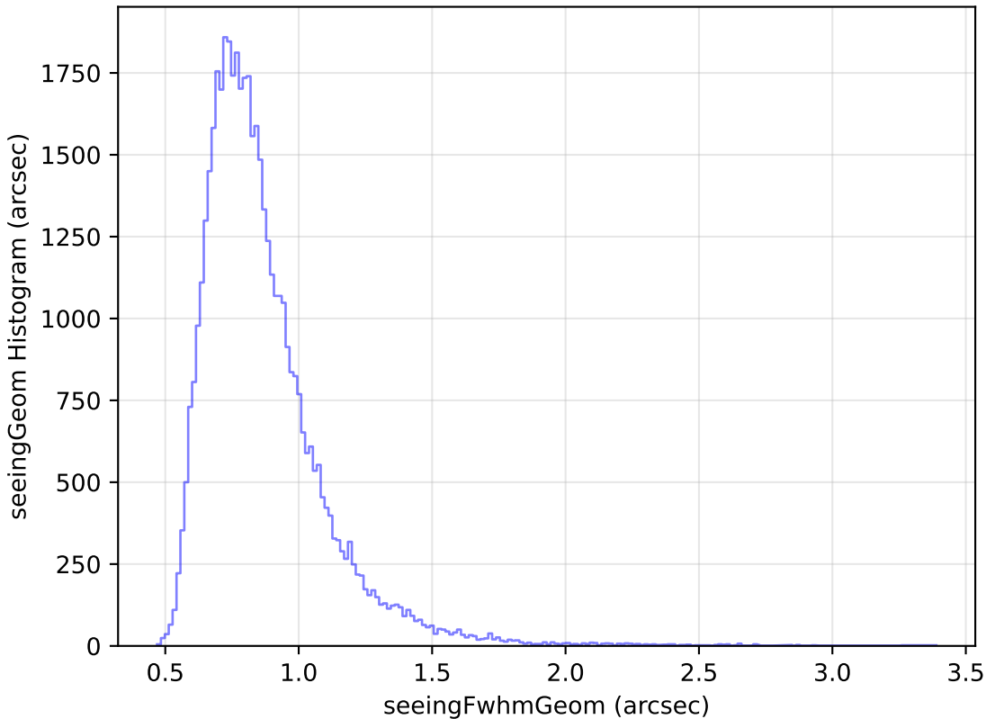
baseline_v2.0_10yrs Yr 1 i band: seeingGeom Histogram
