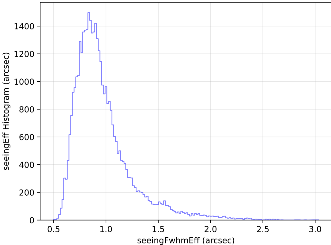
baseline_v2.0_10yrs Yr 1 z band: seeingEff Histogram
