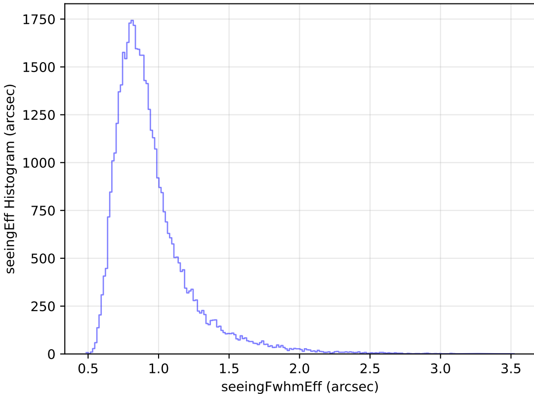
baseline_v2.0_10yrs Yr 1 y band: seeingEff Histogram
